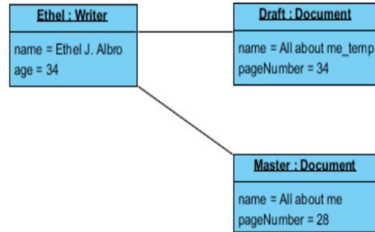
Object Diagram
